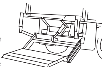
2 Step Gravity Step
